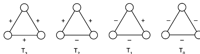
Figure 2 All four possible signed triads, as per Structural Balance Theory. The subscript number following the “T” corresponds to the number of positive connections for that triad
